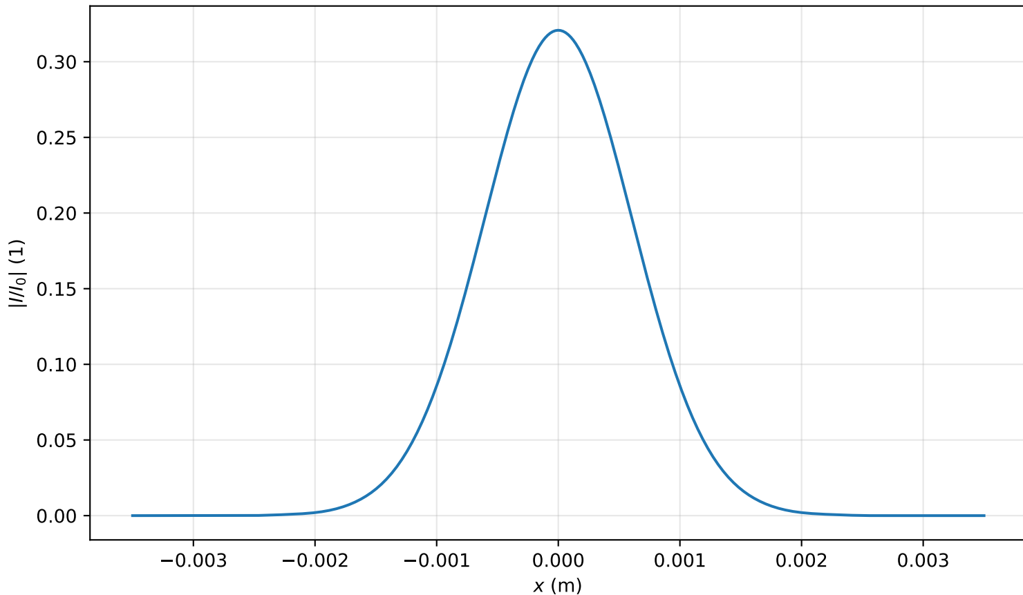
Intensity profile I(x, y = 0, z = 3.105m)/I_0 , P_{in}=0.1P_{cr} , artificial time
